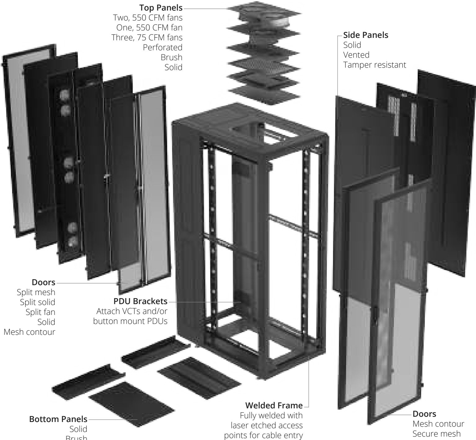
84"H x 30"W x 42"D frame shown, six top cabinet knockouts are part of 30/32" frames only
