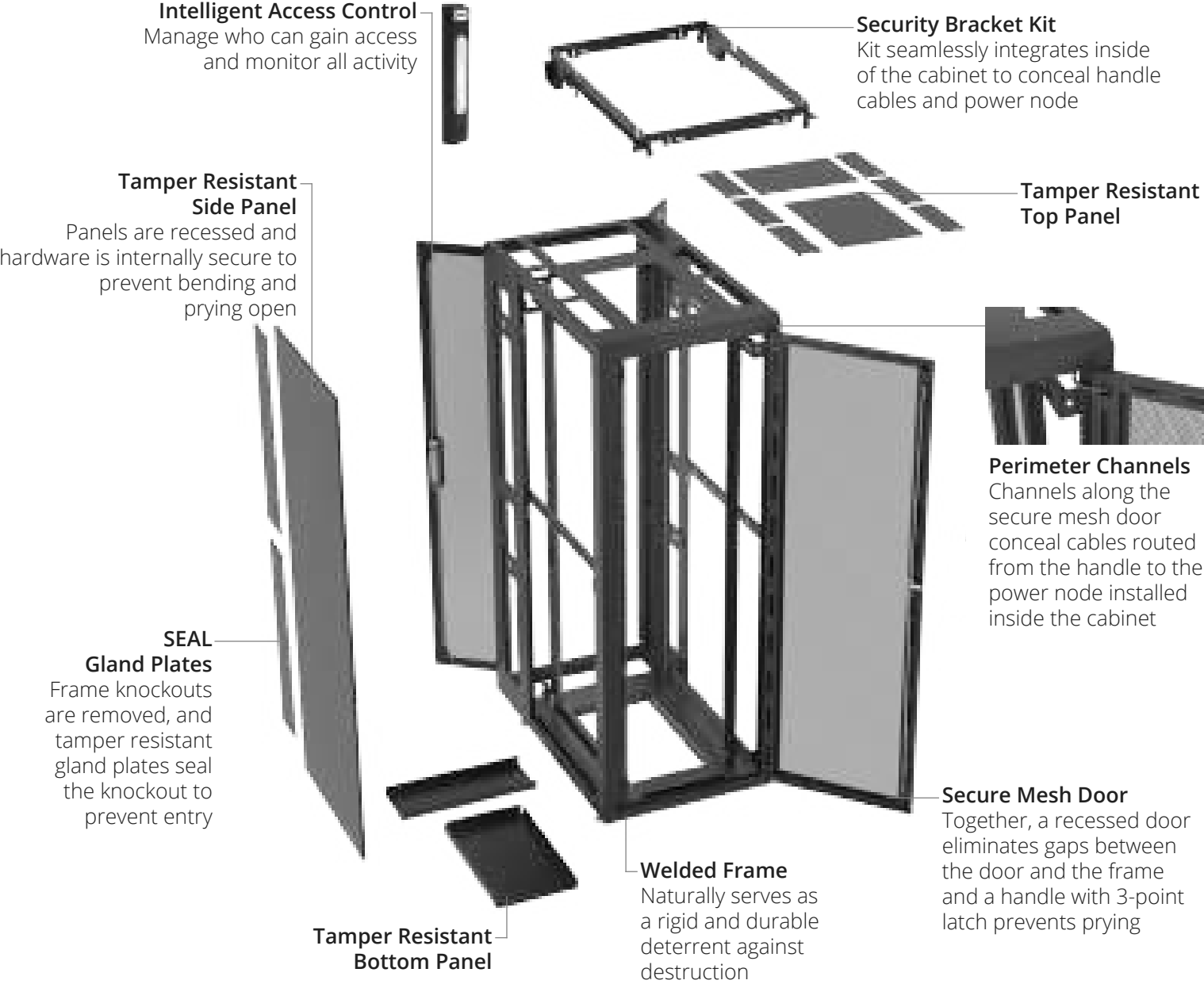
84"H x 30"W x 42"D frame shown, six top cabinet knockouts are part of 30/32" frames only
