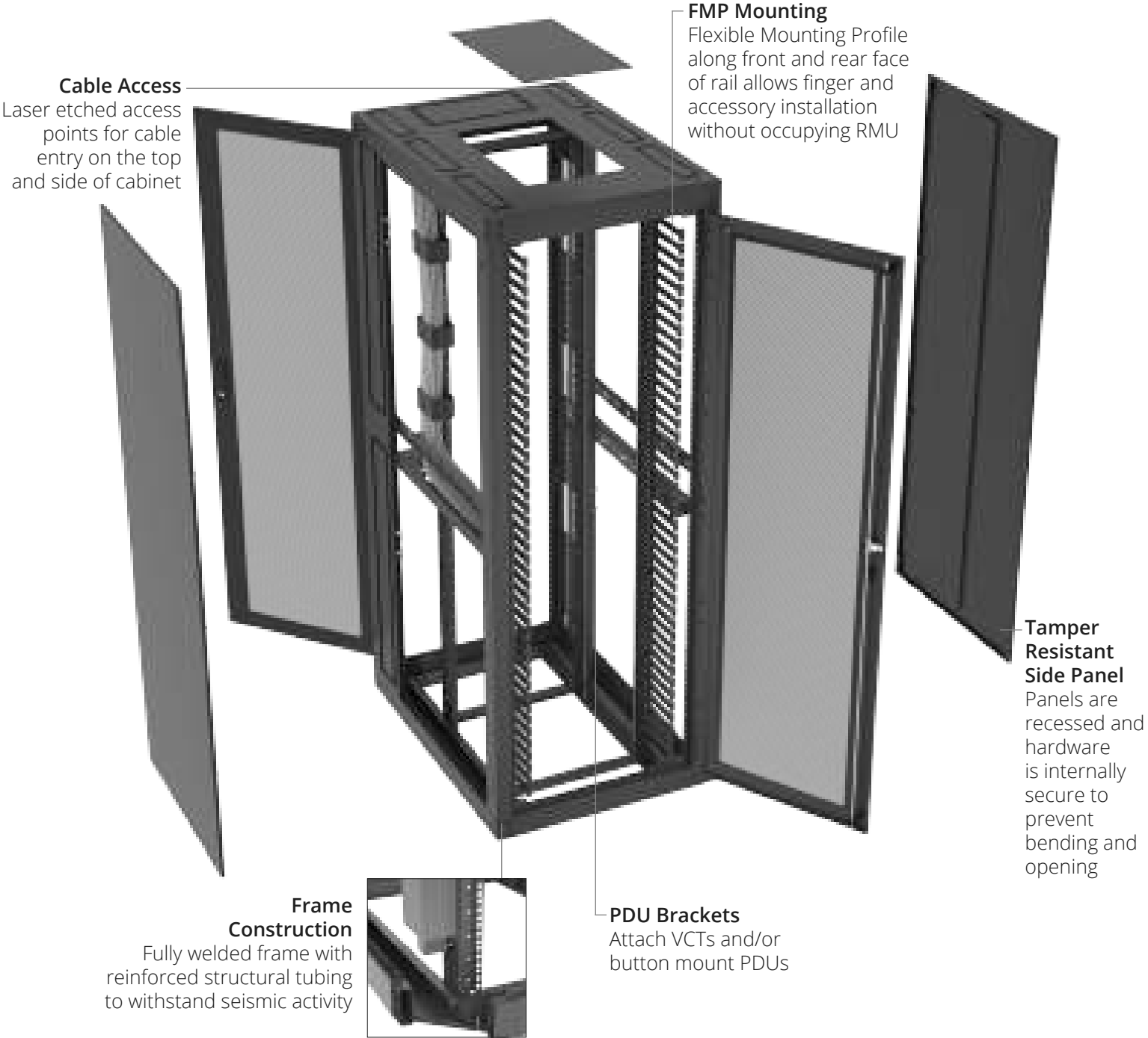
84"H x 30"W x 42"D frame shown, six top cabinet knockouts are part of 30" frames only
