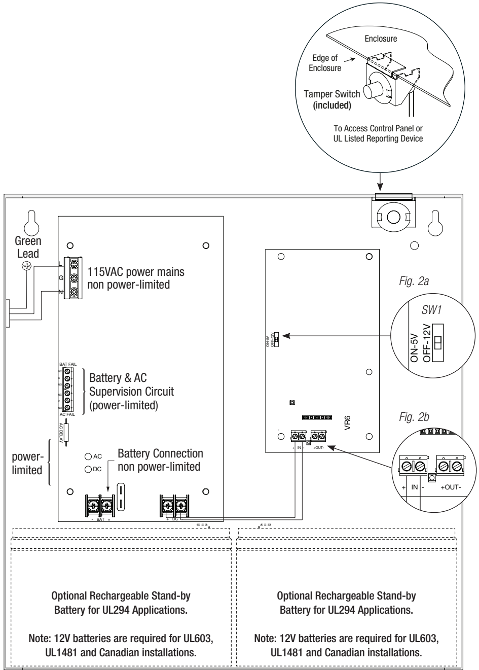
Fig. 2 - AL1024NK1 Configuration
