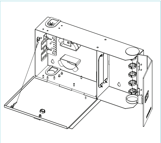
PWH-02P (accepts up to 2 CCH panels) | Drawing ZA-3078
