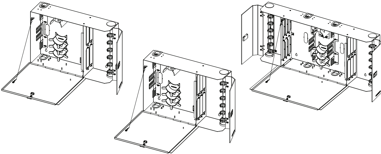
PWH-04P (accepts up to 4 CCH panels), PWH-06P (accepts up to 6 CCH panels) and PWH-12P (accepts up to 12 CCH panels) (shown left to right) | Drawing ZA-3453
