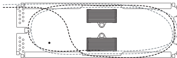
24-Position RTV Splice Closure | Drawing ZA-2270
