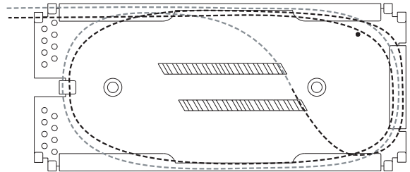
12-Position Heat-Shrink Splice Closure | Drawing ZA-2273
