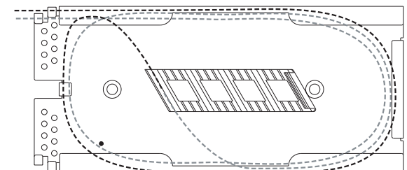
24-Position Heat-Shrink Splice Closure | Drawing ZA-2274
