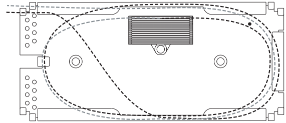
12-Position RTV Splice Closure | Drawing ZA-2271
