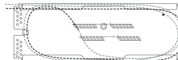
12-Position Mechanical Splice Closure | Drawing ZA-2269
