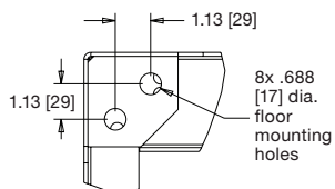
detail A for DRK, MRK, WRK Series
